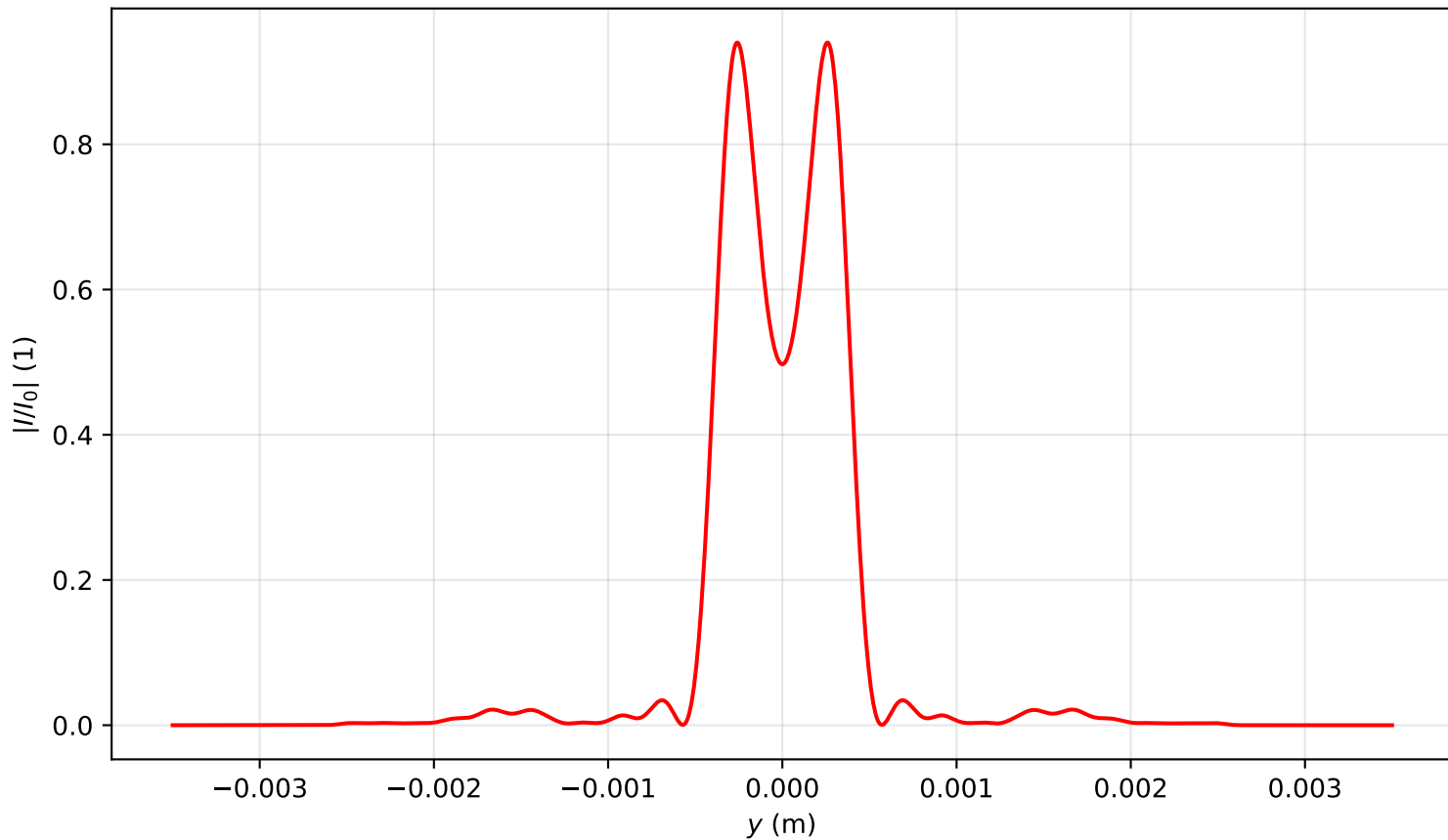
Intensity profile I(x=0, y, z=2.388)/I_0 , \text{Pin}=2.5\text{Pcr} , artificial time
